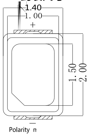
Fig.1-1 Top View
