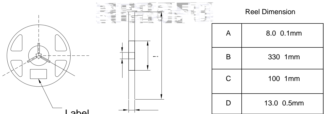
Fig.2-2 Reel Dimension
