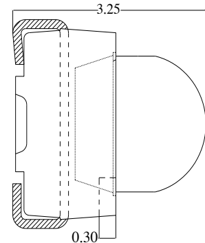
Fig.1-2 Side View
