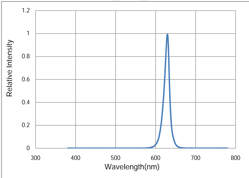
Fig. 1-14 Spectrum Distribution
