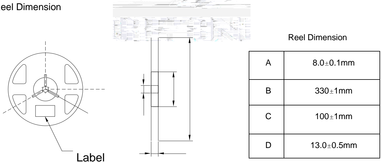
Fig.2-2 Reel Dimension
