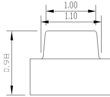
Fig.1-2 Side view
