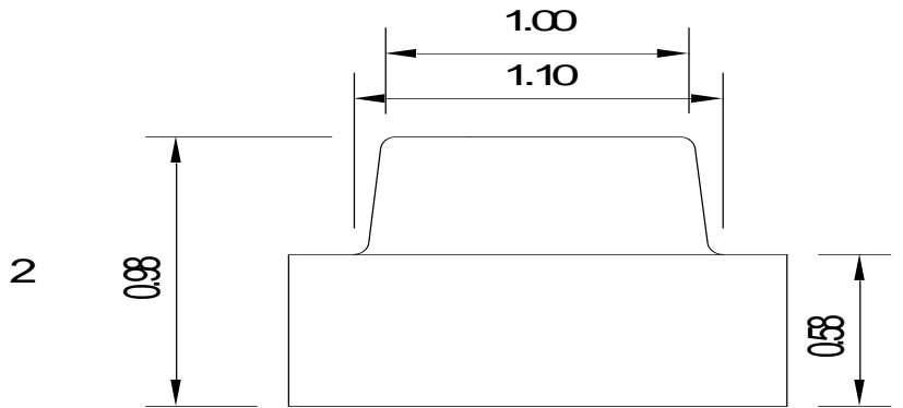
Fig.1-2 Side view
