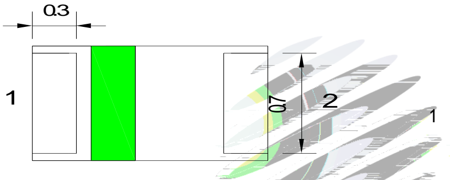
Fig.1-3 Bottom view
