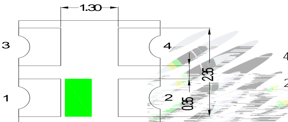
Fig.1-3 Bottom view
