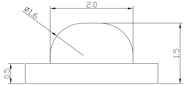
Fig.1-2 Side view 使
