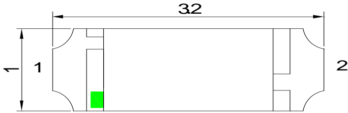
Fig.1-1 Top view
