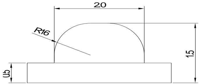
Fig.1-2 Side view
