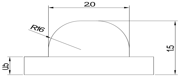
Fig.1-2 Side view
