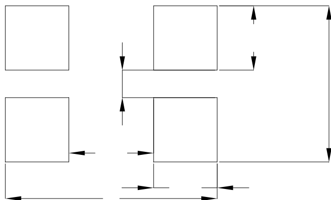
Fig.1-5 Soldering patterns
