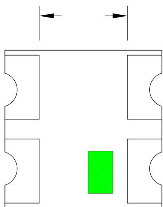
Fig.1-3 Bottom view
