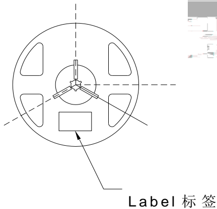
Fig.2-2 Reel Dimension
