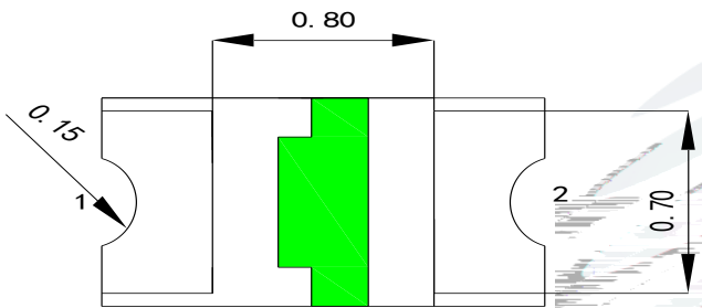
Fig.1-1 Top view
