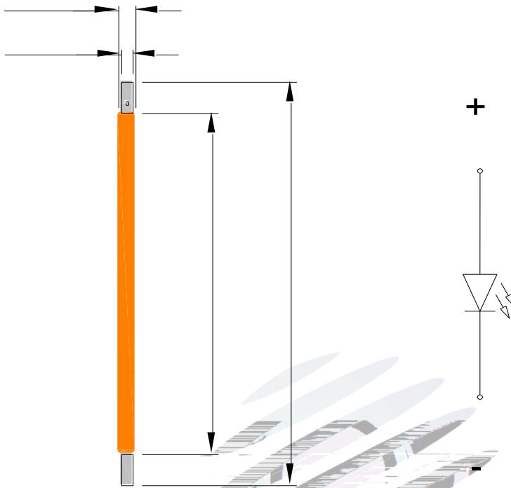
Fig.1-1 Top View
