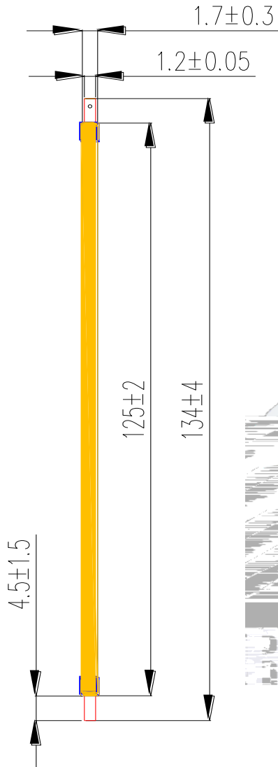
Fig.1-1 Top view
