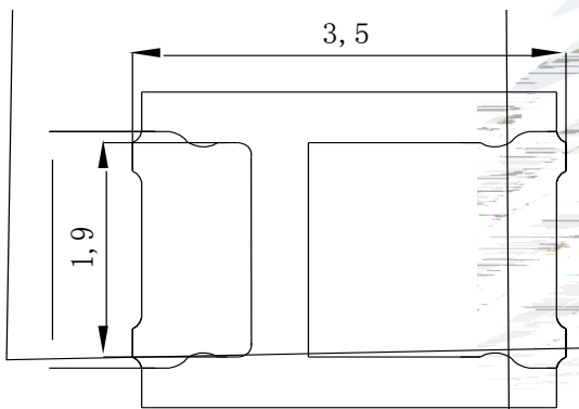
Fig.1-3 Bottom view
