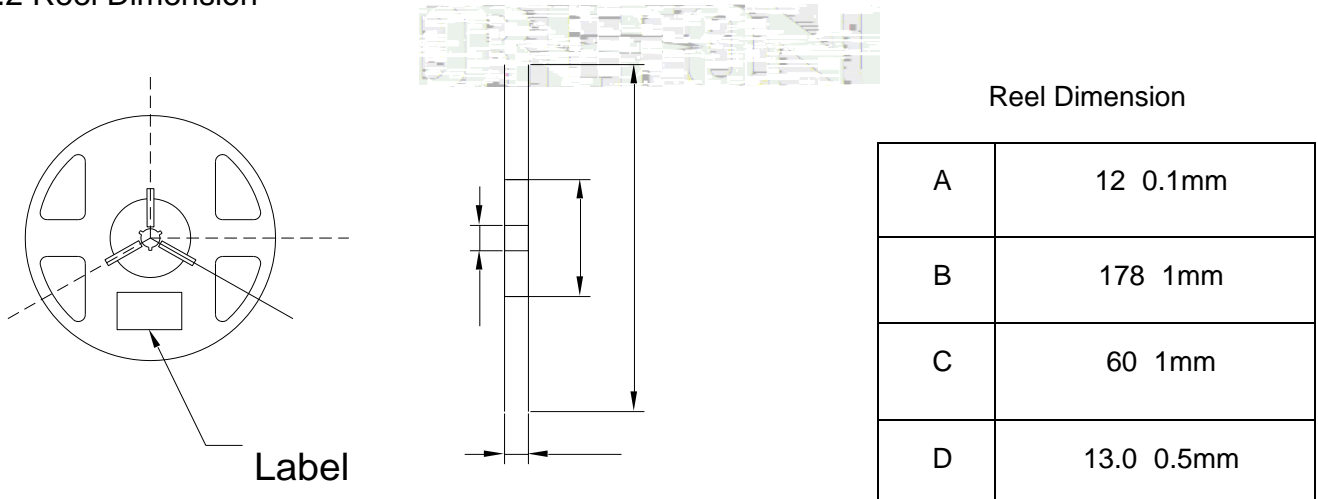
Fig.2-2 Reel Dimension
