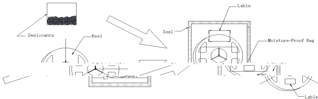
Fig.2-4 Moisture Resistant Packing
