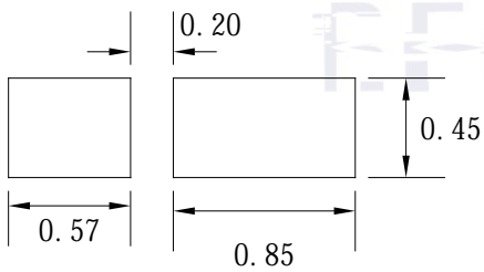
Fig 1-5 Soldering Patterns
