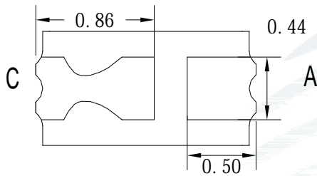
Fig 1-3 Bottom View
