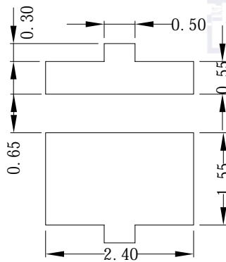
Fig.1-5 Soldering Patterns
