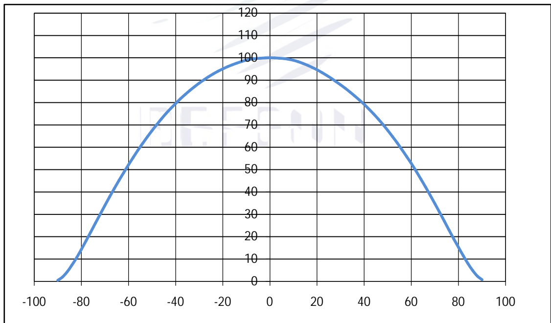
Fig. 1-12 Radiation diagram
