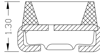
Fig. 1-2 Side view
