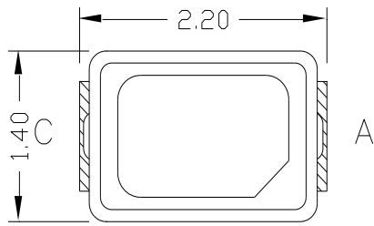
Fig. 1-1 Top view
