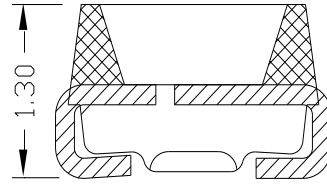
Fig. 1-2 Side view
