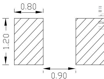
Fig. 1-5 Soldering patterns
