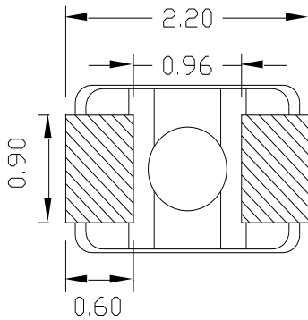
Fig. 1-3 Bottom view
