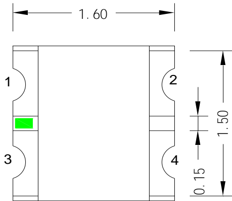
Fig.1-1 Top view
