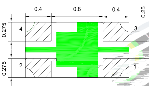
Fig.1-3 Bottom view
