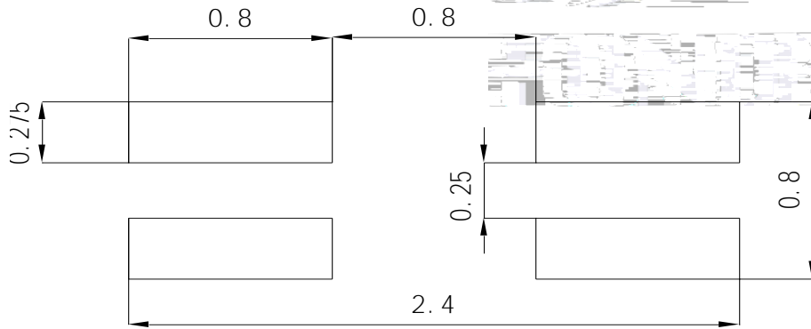
Fig.1-5 Soldering patterns
