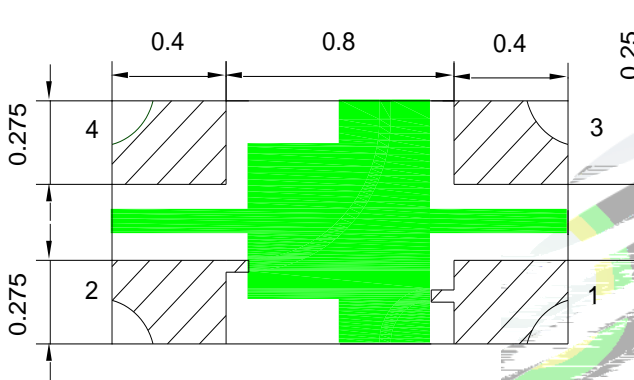
Fig.1-3 Bottom view
