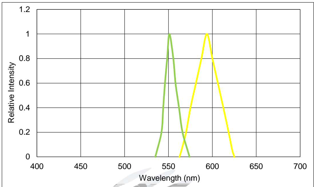
Fig.1-12 Relative Intensity Vs Wavelength (Ta=25 )
