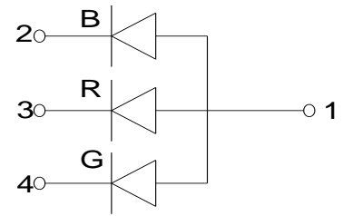
Fig.1-4 Polarity
