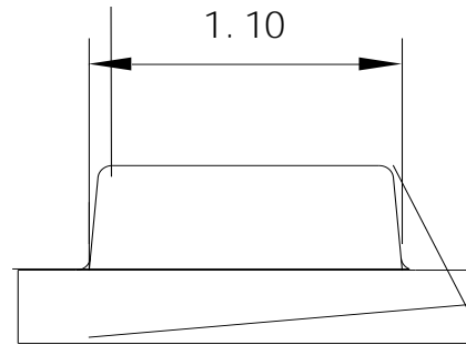
Fig.1-2 Side view
