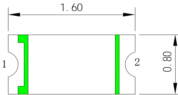
Fig.1-1 Top view
