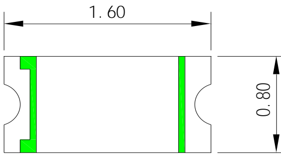
Fig.1-1 Top view
