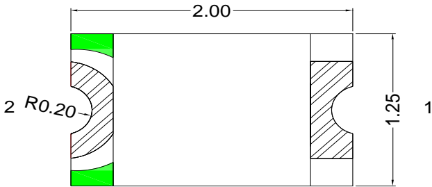
Fig.1-1 Top view
