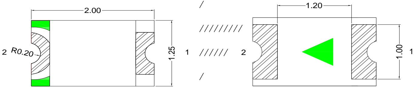
Fig.1-1 Top view/
