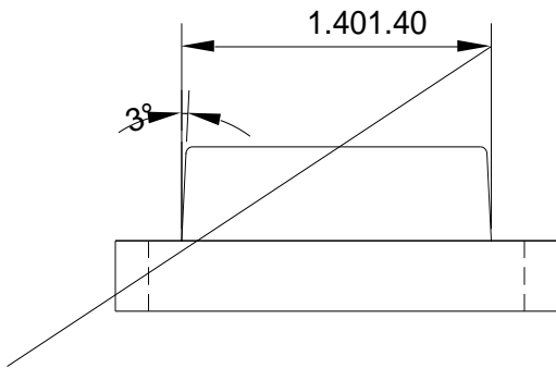
Fig.1-3 Side view
