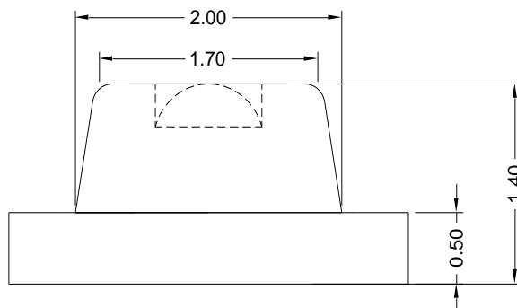
Fig.1-2 Side view
