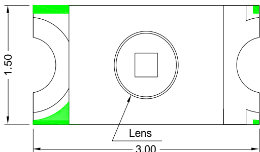
Fig.1-1 Top view
