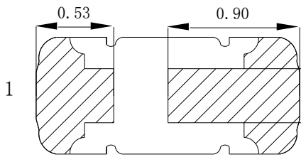
Fig.1-3 Bottom view
