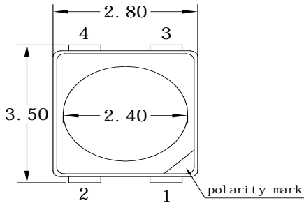
Fig. 1-1 Top View
