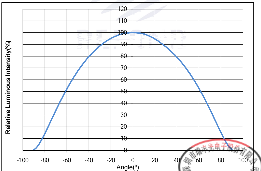
Fig. 1-12 Radiation diagram
