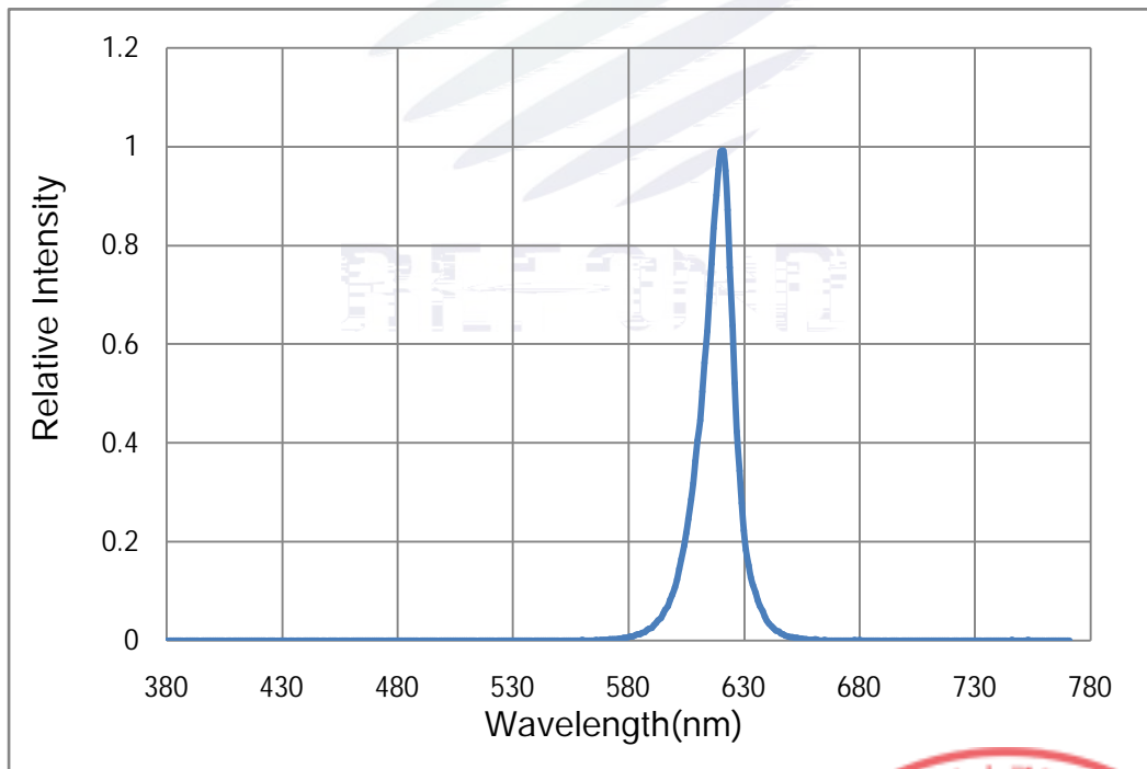
Fig. 1-14 Spectrum Distribution
