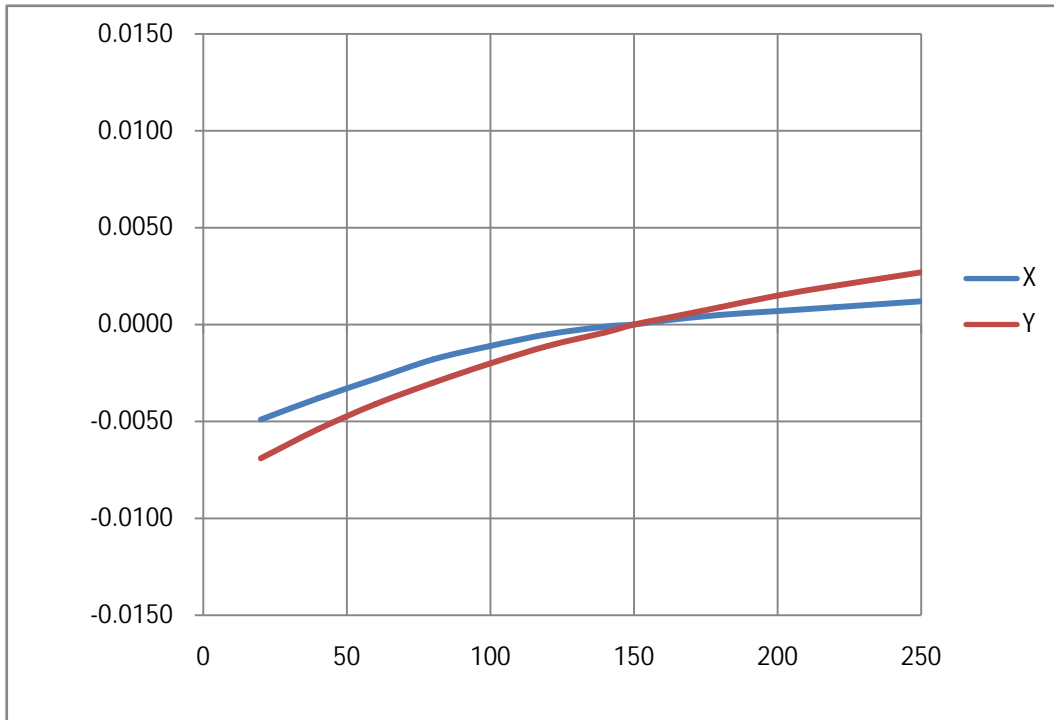
Fig. 1-13 Chromaticity Coordinate Vs Forward Current
