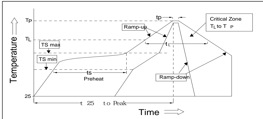
Fig.3-1 SMT Reflow Soldering Instructions SMT 5 [(c0-9PE
