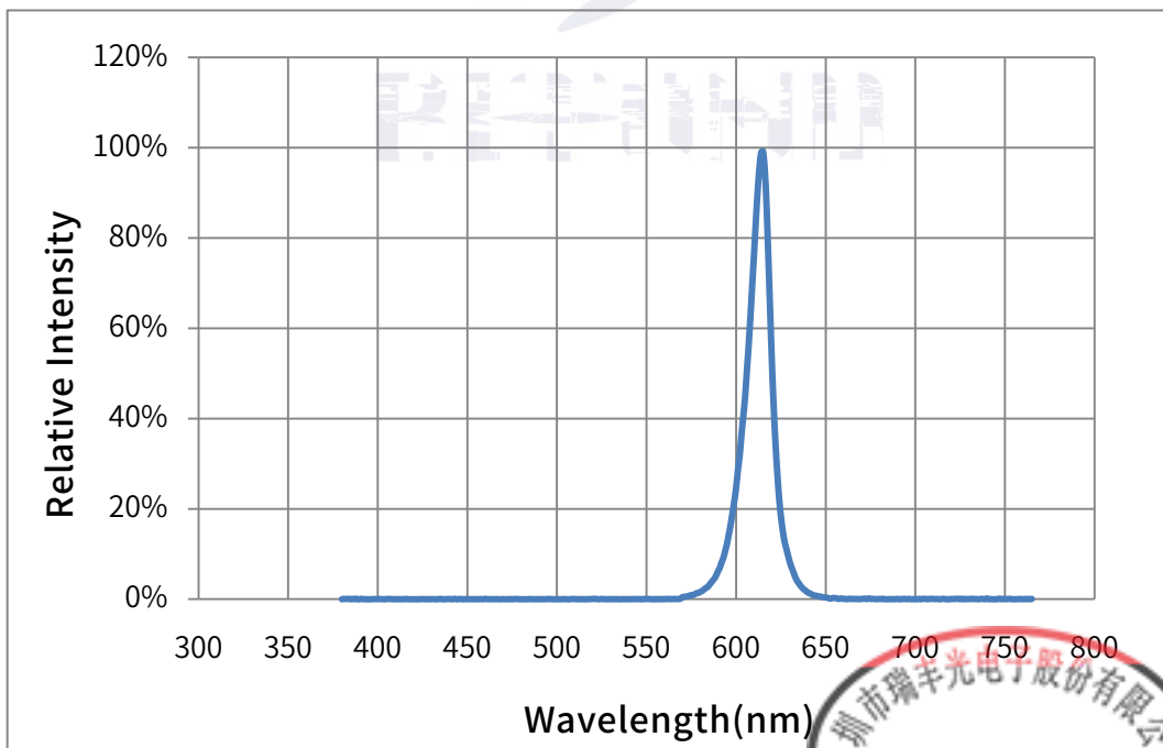
Fig. 1-14 Spectrum Distribution
