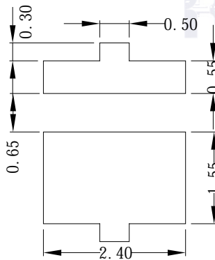
Fig.1-5 Soldering Patterns
