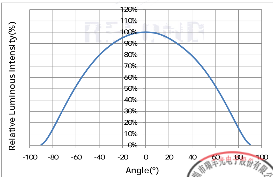
Fig. 1-12 Radiation diagram
